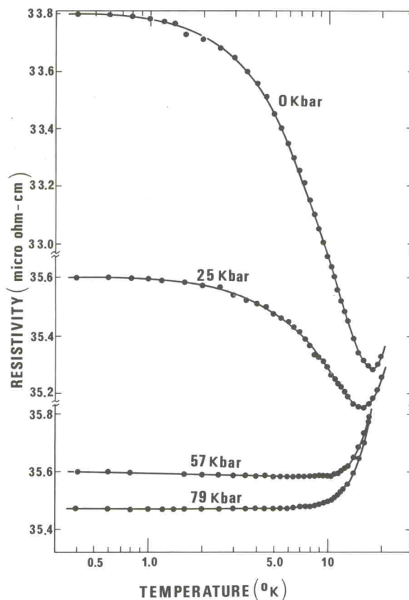
FIGURE 5 Resistivity versus temperature of YCe (1 at. % Ce) at various pressure up to 79 kbar (reference 12).
